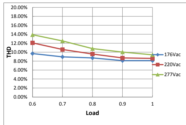
THD Curve
