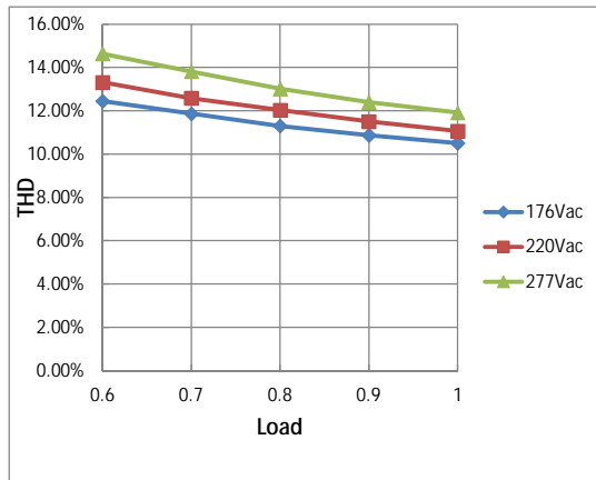
THD Curve
