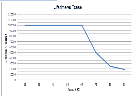
LIFETIME Curve
