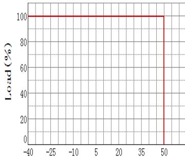
Derating Curve
