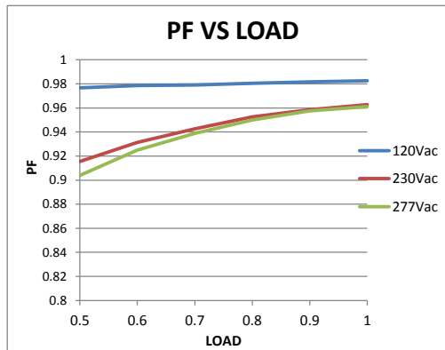
Power Factor VS. Load Curve(Model:12A)
