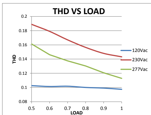
THD VS. Load Curve(Model:12A)
