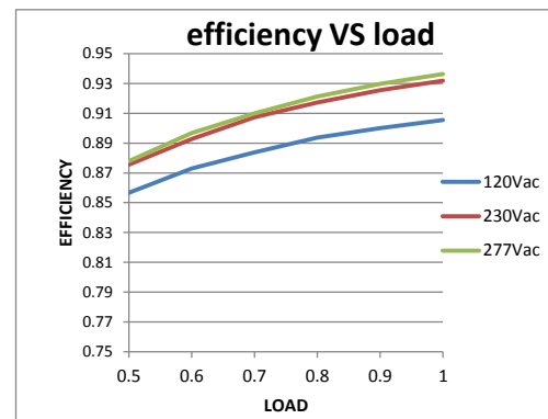
Efficiency VS. Load Curve(Model:12A)
