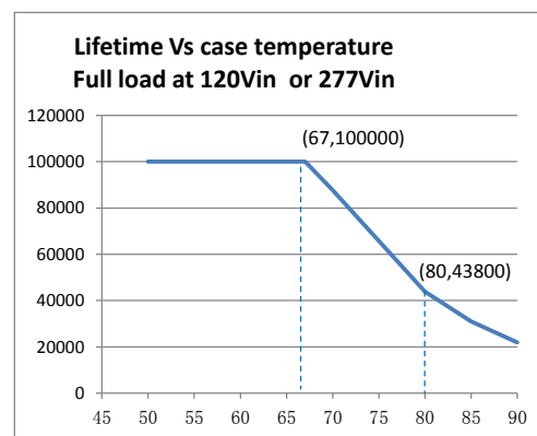
Life Time VS. Tcase (Ref.)(Model:12A)
