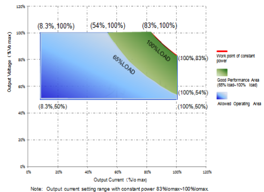
V/I Operating Area
