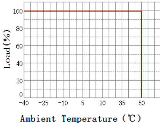
Derating Curve
