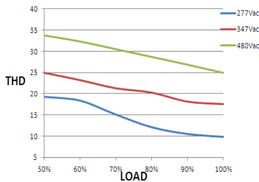
THD VS. Load Curve
