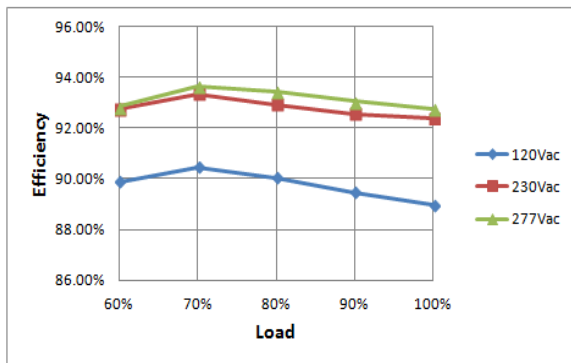
Efficiency VS. Load Curve (700mA)
