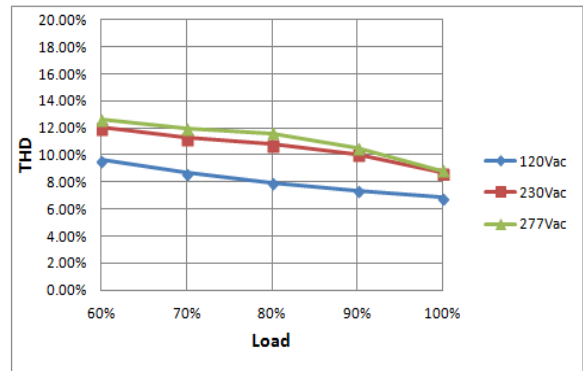
THD Curve
