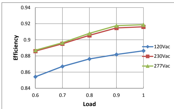
Efficiency VS. Load Curve (typ.)
