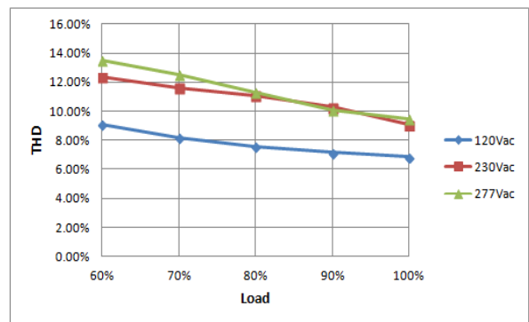
THD Curve
