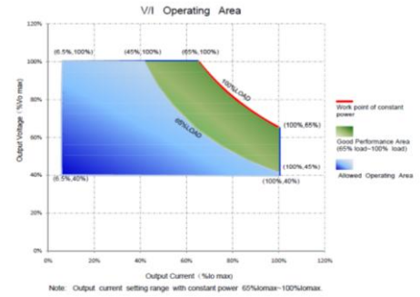
V/I Curve
