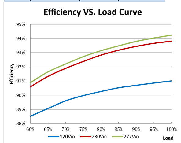
Efficiency VS. Load Curve(Model:700mA)
