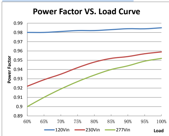
Power Factor VS. Load Curve
