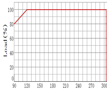
Derating Curve
