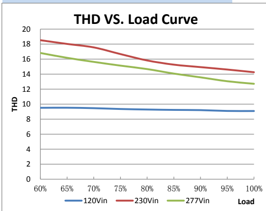
THD VS. Load Curve
