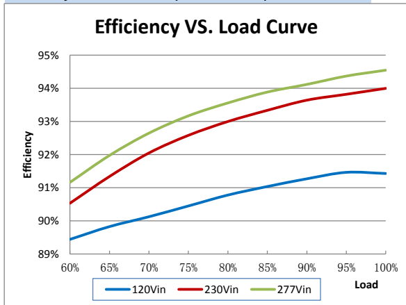
Efficiency VS. Load Curve(Model:850mA)
