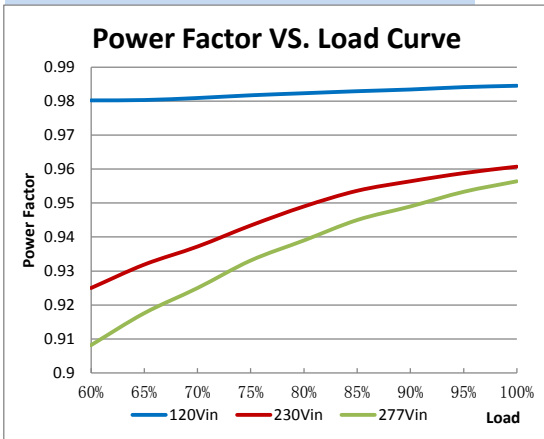
Power Factor VS. Load Curve
