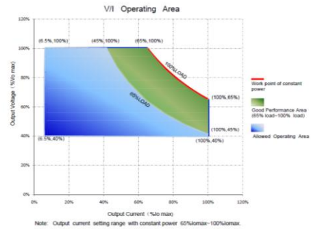
V/I Curve
