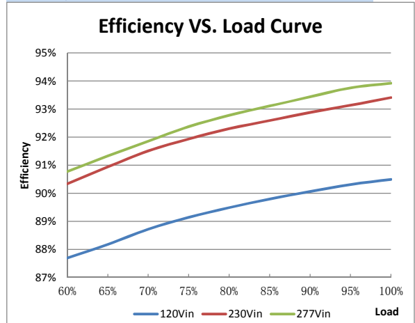
Efficiency VS. Load Curve(Model:1.3A)
