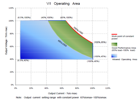
V/I Curve
