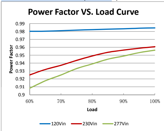
Power Factor VS. Load Curve(Model:4.8A)
