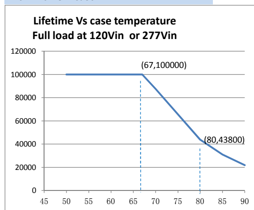
Life Time VS. Tcase
