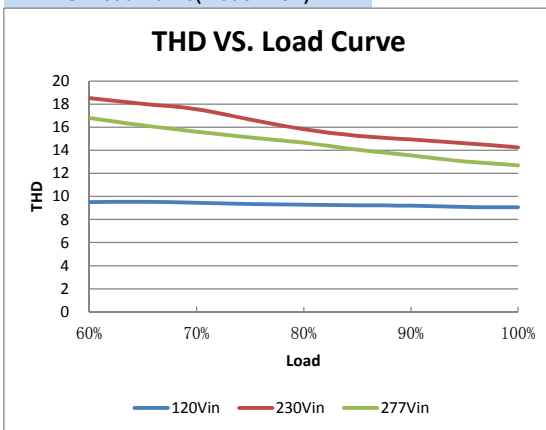
THD VS. Load Curve(Model:4.8A)
