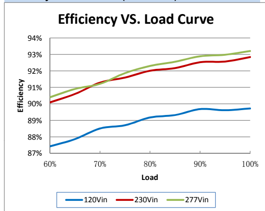
Efficiency VS. Load Curve(Model:4.8A)
