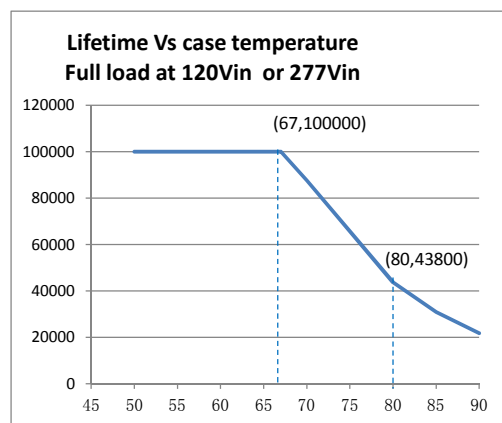
Life Time VS. Tcase (Ref.)(Model:6.8A)
