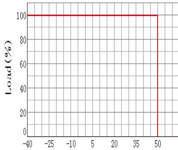
Derating Curve
