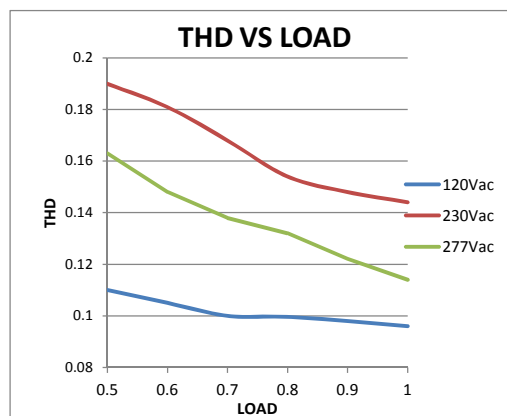
THD VS. Load Curve(Model:6.8A)
