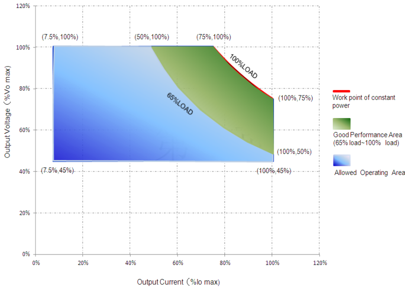
V/I Operating Area
